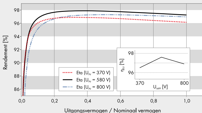
Rendementscurve SUNNY TRIPOWER 10000TL
